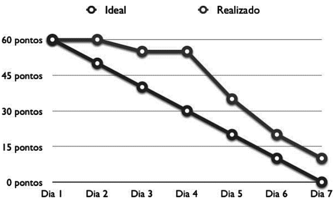
Figura 5.1: Burndown Chart
