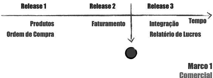
Figura 3.8: Roadmap
