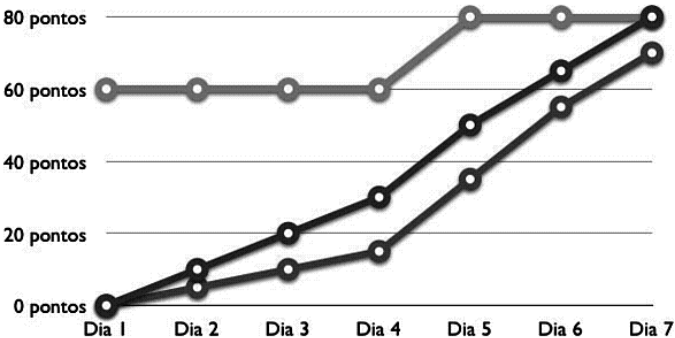
Figura 5.2: Burnup Chart
